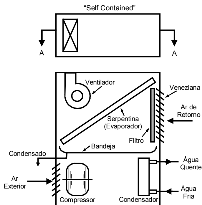
Figura 6.15: Condicionador Self-Contained.
